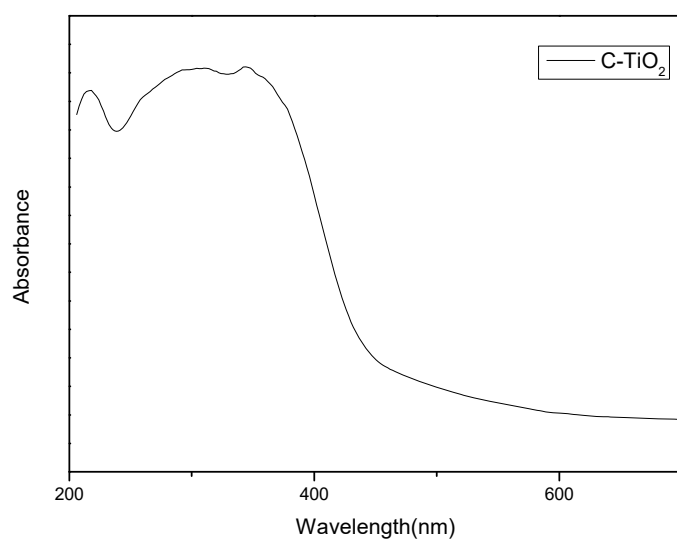
Fig. S1. UV-vis diffuse reflectance absorption spectrum of C-TiO 2
