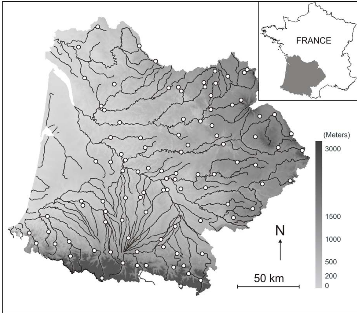
Fig. S1. Location of the 100 sampling sites in the Adour-Garonne stream system (south-western France).
