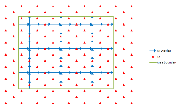
Figure 1. Typical layout of a portion of an ORION 3D omnidirectional survey. Receiver dipoles are shown as blue arrows, current injection points as red triangles.
